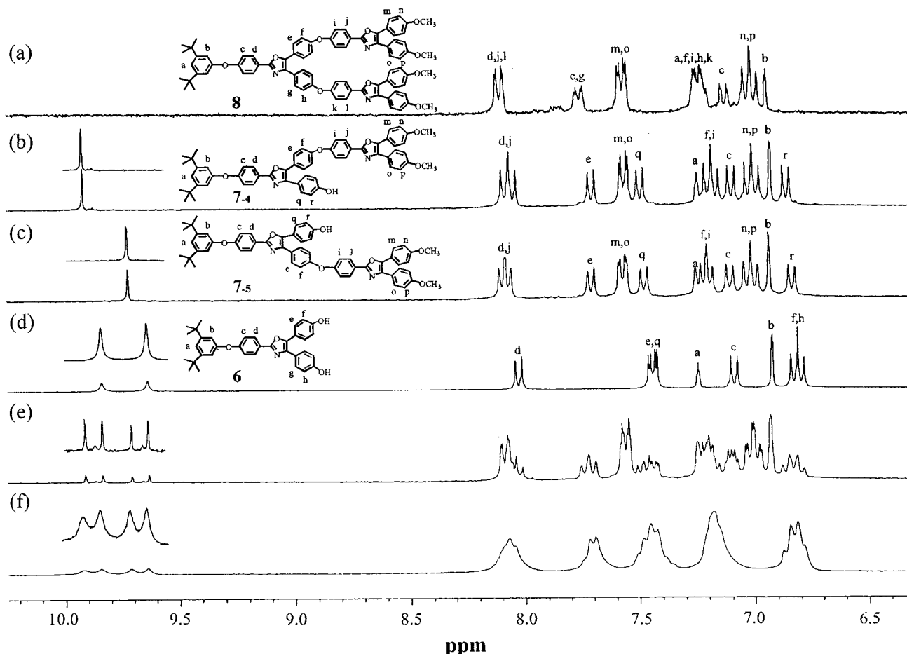
Figure 3. ^1\text{H} NMR spectra in \text{DMSO}-d_6 of model compounds (a) 8 , (b) 7-4 , (c) 7-5 , (d) 6 , and (e) the reaction mixture obtained directly from the model reaction without further separation, compared with (f) the hyperbranched poly(aryl ether oxazole) P1 .
