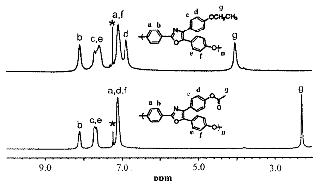
Figure 4. 1 H NMR spectra in CDCl 3 of the hyperbranched poly(aryl ether oxazole)s P2 and P4 . Asterisk: signal due to CDCl 3 .
